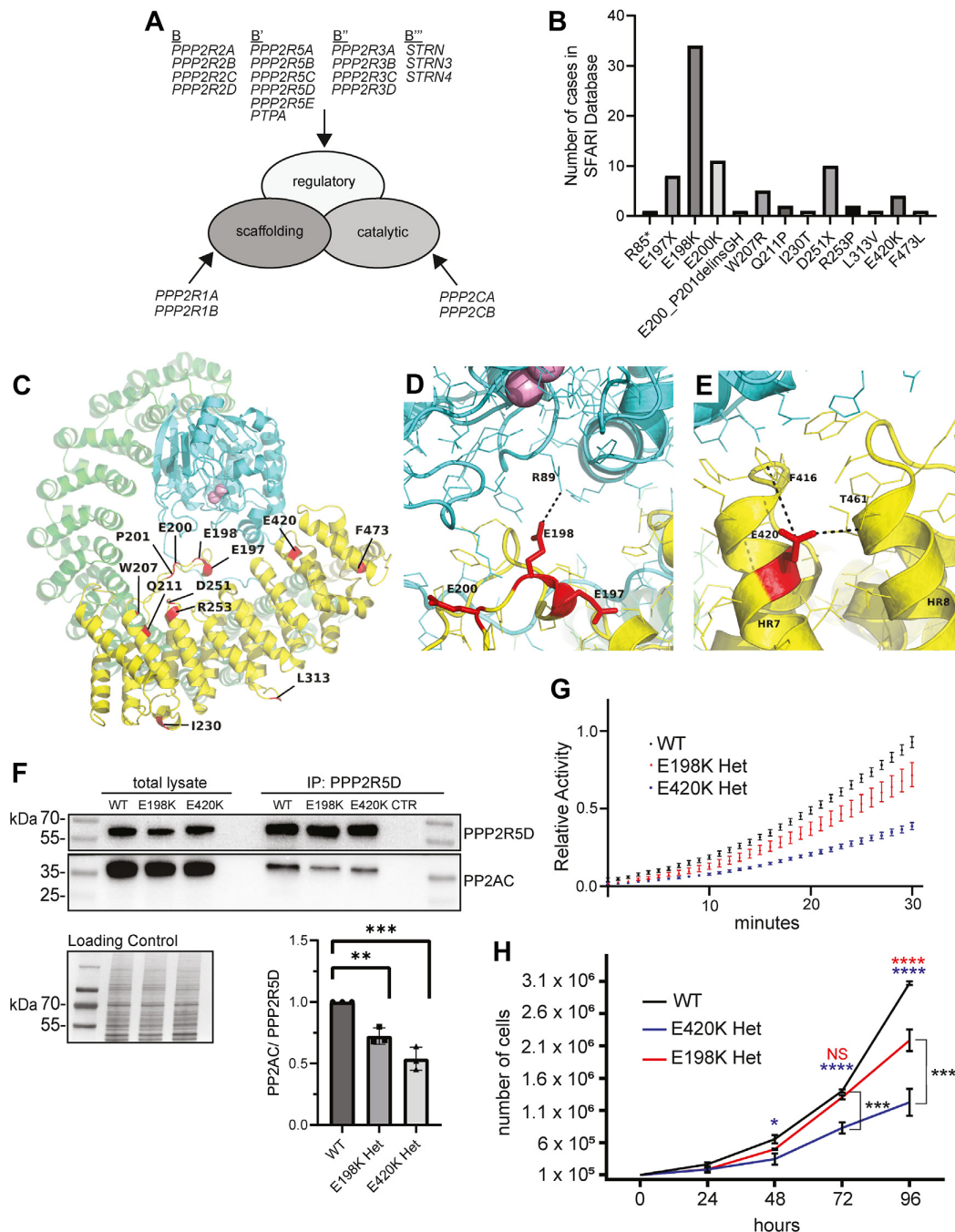
Figure 1. PP2A holoenzyme structure, PPP2R5D variants, and E198K versus E420K variant activity profiling. A, diagram of PP2A holoenzyme structure and components. B, number of cases corresponding to pathogenic PPP2R5D variants based on SFARI database. C, homology model of the PP2A holoenzyme containing PPP2R5D showing the locations of the common PPP2R5D variants. This PPP2R5D model is superimposed onto the known structure of the PPP2R5C-containing holoenzyme (PDB ID: 2IAE). PPP2R5D is colored in yellow, the scaffold subunit in green, and the catalytic subunit in cyan. Metal ions of the catalytic site are pink spheres. Red surfaces correspond to the variant sites such as E198 and E420. D, a zoomed in view of E198 shows an interaction with R89 of the catalytic subunit. E, a zoomed in view of E420 shows potential interactions with aromatic ring hydrogens of F416 and the sidechain of T461. F, Western analysis of total cell lysates (input) and endogenous PPP2R5D IPs probed for PPP2R5D or for the PP2A catalytic subunit (PP2AC). Relative amounts of PP2AC from WT, E198K-het, or E420K-het cells normalized to total PPP2R5D in IPs and represented as the mean percent of WT. The control (CTR) is bead only. Coomassie stain was used as a loading control. (N = 3 independent biological replicates, mean \pm SD, * p < 0.05, ** p < 0.01, *** p < 0.001) G, relative phosphatase activity of endogenous PPP2R5D IPs. Endogenous PPP2R5D was immunoprecipitated from WT, E198K-het, and E420K-het cells, and hydrolysis of DiFMUP was measured at Ex 360 nm and at Em 460 nm. Activity was normalized to total levels of PPP2R5D detected in IPs through immunoblotting shown in (F). WT activity (black) was normalized at 30 min (endpoint) to 1, and variant activity (E198K-het = red and E420K-het = blue) is shown relative to WT (N = 3 independent biological replicates of cells, each performed as n = 2 technical replicates). Error bars represent the mean \pm SD, two-way ANOVA Tukey's, **** p < 0.0001, *** p < 0.001, ** p < 0.01, * p < 0.05, NS: non-significant). PP2A, phosphoprotein phosphatase 2A; PPP2R5D, phosphoprotein phosphatase 2 regulatory protein 5D.
