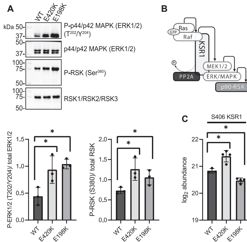
Figure 6. Phosphorylation changes in Ras-MAPK signaling cascade. A, representative immunoblots showing levels of P-p44/p42 MAPK (ERK1/2) T202/Y204 and P-RSK S380 in WT, PPP2R5D E420K-het, and E198K-het HEK293 cell lines. Quantification of P-ERK1/2 (T202/Y204) normalized to total ERK1/2 and of P-RSK (S380) normalized to total level of RSK is shown. B, model depicting KSR1 scaffold leading to coordination of Ras-MAPK signaling following its dephosphorylation of S406 by PP2A. C, LC-MS 3 data for S406 of KSR1 in WT, PPP2R5D E420K-het, and PPP2R5D E198K-het HEK293 cell lines. Value is the log 2 of the TMT intensities detected via LC-MS 3 . For all plots, mean is represented by the column height, and SD is shown in plots as black bars. Statistical significance ( p < 0.05 ) was determined using unpaired, two-tailed t test where an asterisk (*) indicates a significant result. KSR1, Kinase Suppressor of Ras; MAPK, mitogen-activated protein kinase; MS, mass spectrometry; PP2A, phosphoprotein phosphatase 2A; PPP2R5D, phosphoprotein phosphatase 2 regulatory protein 5D; TMT, tandem mass tag.
