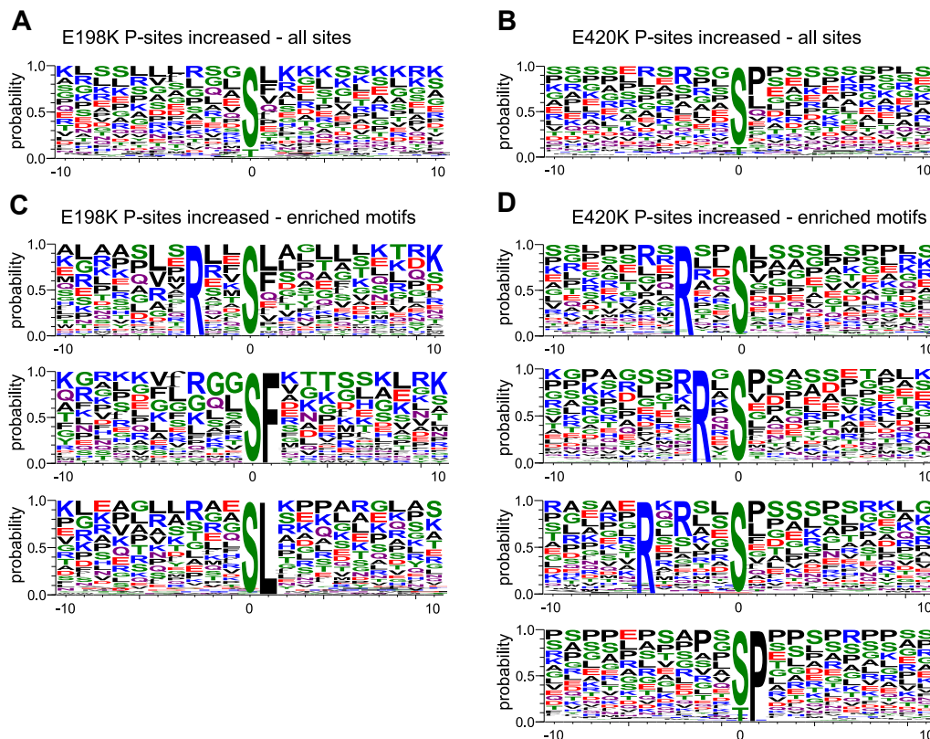
Figure 3. Phosphorylation site motif enrichment analysis of sites that were significantly increased in the E198K and E420K variant cell line. A, weblogs showing enrichment of amino acids surrounding the phosphorylated residue for sites significantly increased by at least two-fold in PPP2R5D E198K (A) and E420K (B) variant cells. C, enriched motifs among significantly increased phosphorylation sites in the E198K variant. D, enriched motifs among significantly increased phosphorylation sites in the E420K variant. PPP2R5D, phosphoprotein phosphatase 2 regulatory protein 5D.
